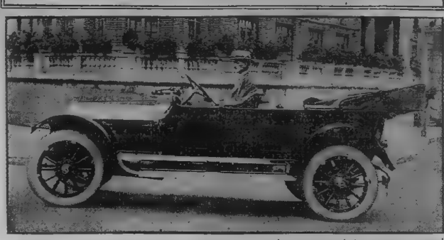
A 4-cylinder model touring car. Features include 45-horse-power en bloc motor, 122-inch wheel base, vacuum gasoline feed, high tension magneto, one-man top, rain vision shield, left-hand drive, center control, seats seven passengers, streamline body. This car is now on display at the Overland Southern show room on Peachtree street.
